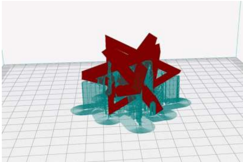
Figure 6. Setting up a stand for proper printing of the object
