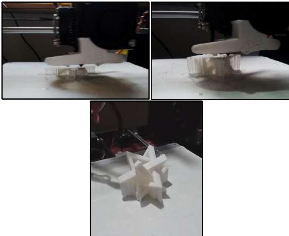
Figure 7. Printing of the model in all phases
