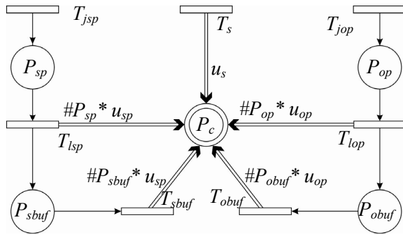
Figure 4. FSPN model with buffering
