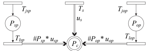
Figure 1. Basic FSPN model of P2P live video streaming system
