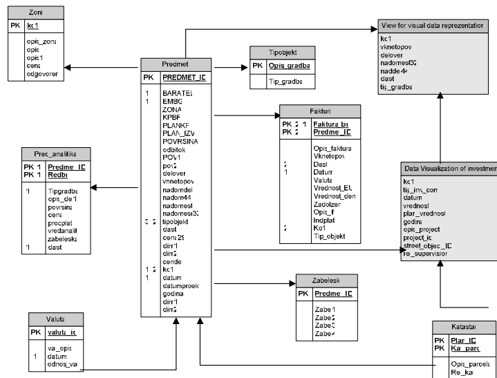
Fig 3 An Example of ER diagram of the bases of one of the services in the local government- the Division of Communal Affairs in the Department of Urbanism, Ecology and Communal Works within Local Government
