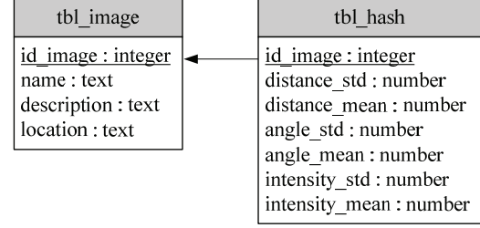
Fig. 3. Relations schema for the database with images.
