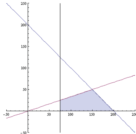
Figure 2. The feasible region of Problem 4.
