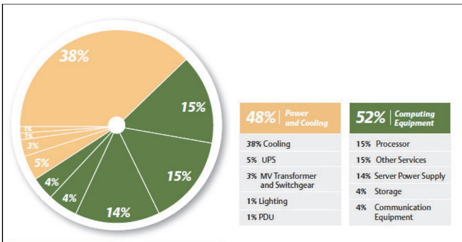
Fig. 1 Data-com equipment accounts for over 50% of the energy used while power and cooling account for an additional 48% in a traditional data centre
