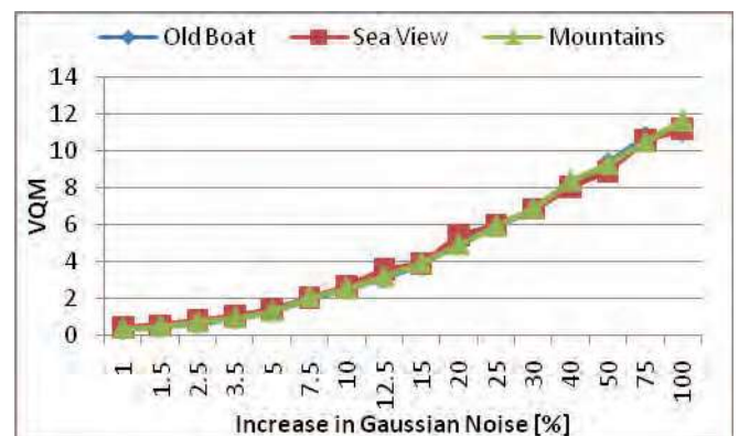
Fig. 10. VQM increase due to the amount of Gaussian noise
