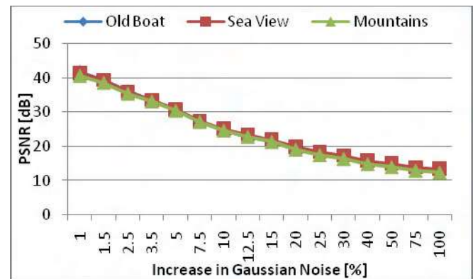
Fig. 4. PSNR decrease due to the amount of Gaussian noise.
