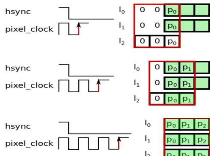
Fig. 4. Realization of the Sobel Sliding Window
